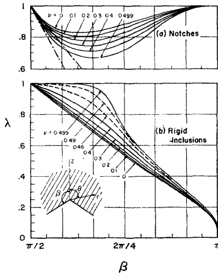
Fig. 2. The smallest value of \lambda in axisymmetric elastic problems.
